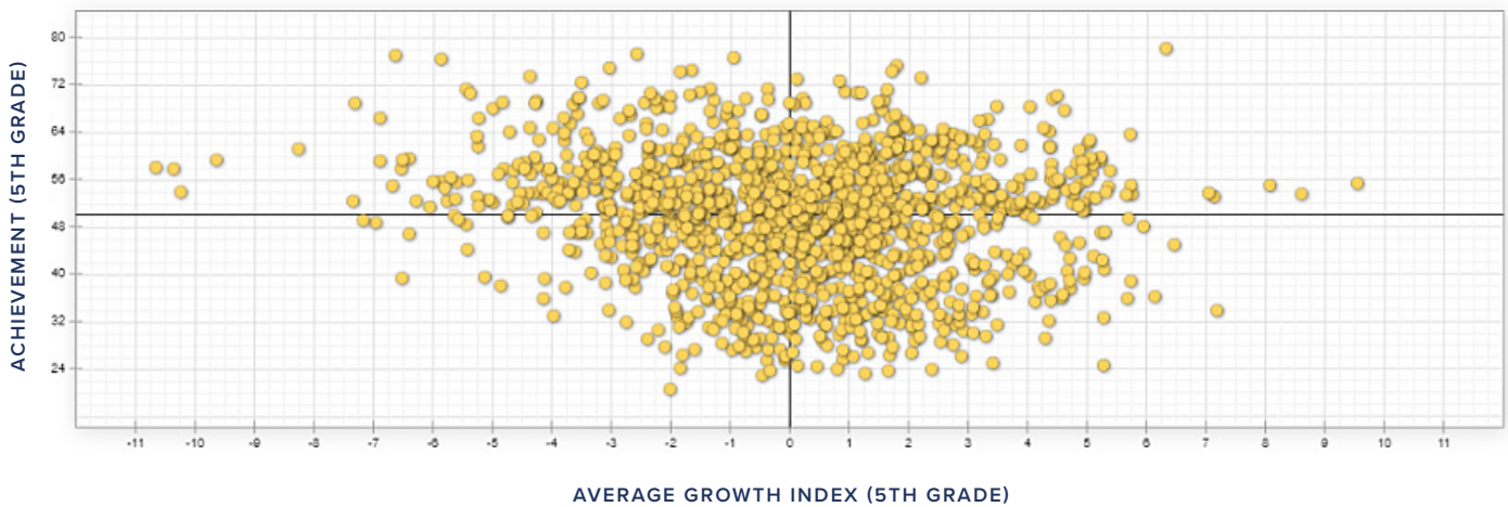
School Scatterplot
