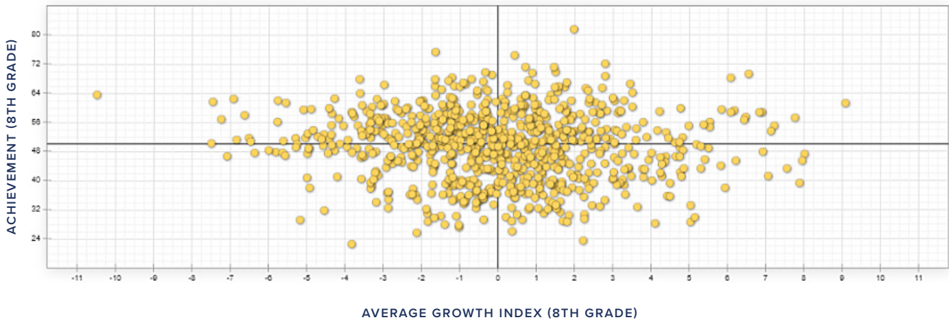
School Scatterplot
